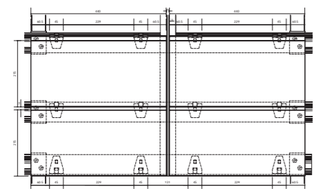
General Assembly Front Elevation (Not to scale)
